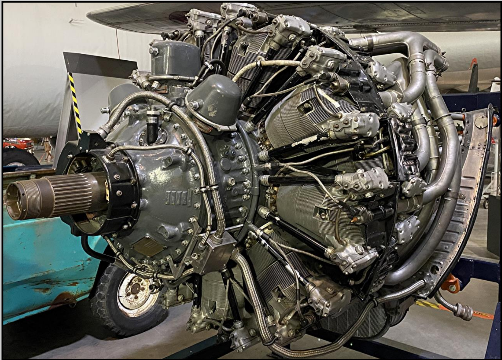
This R-2800 Double Wasp Radial Engine is located at the Strategic Air Command Air and Space Museum located near Omaha, Nebraska.
